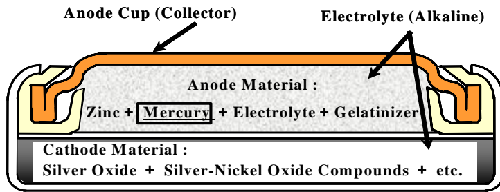
Fig. 1. Schematic Diagram of Silver Oxide Battery Cell
