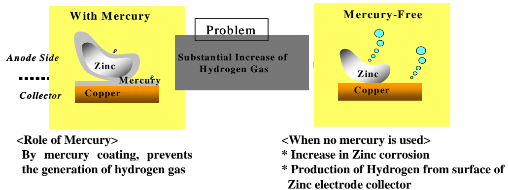
Fig 2. Role of mercury in conventional silver oxide battery cell
